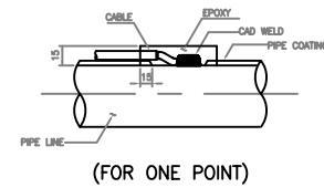
DETAIL 3 BONDING CADWELD
