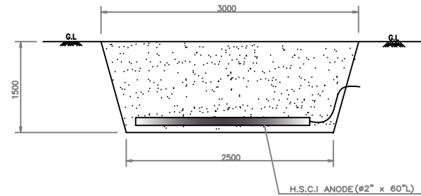
DETAIL 5 ANODE INST
