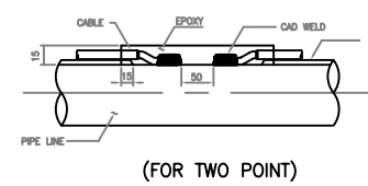
DETAIL 3 BONDING CADWELD
